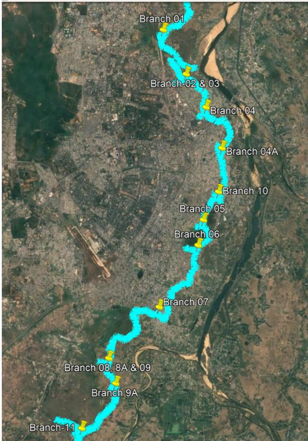
Flow calculation locations at branches for Float method
