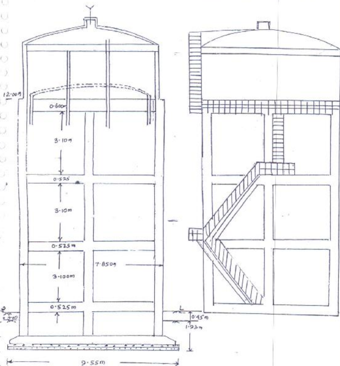
FRONT ELEVATION
