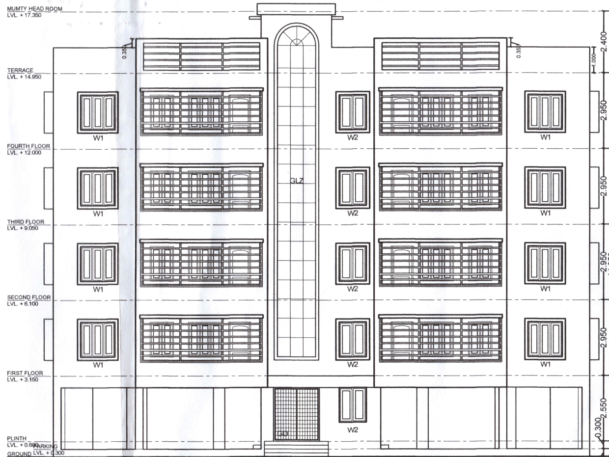
FRONT ELEVATION
