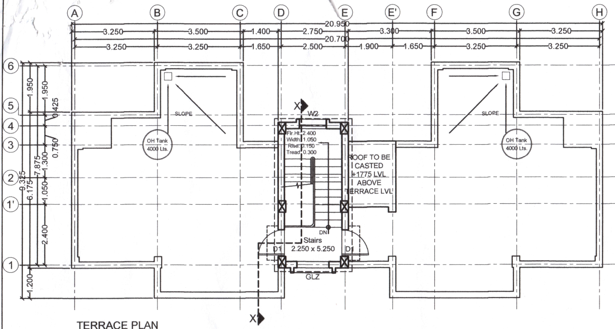
TERRACE PLAN
