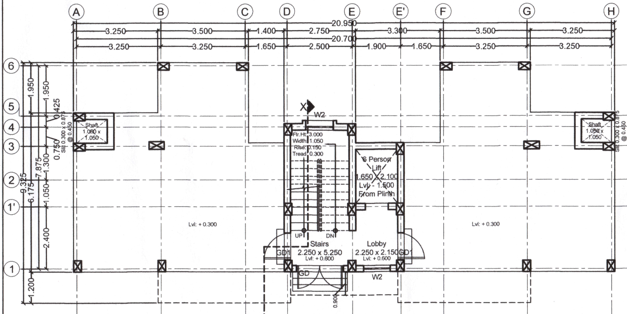
STILT PLAN
