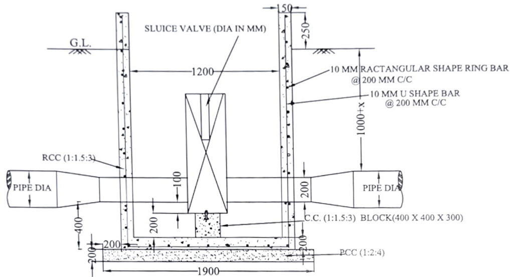
SECTION X-X
