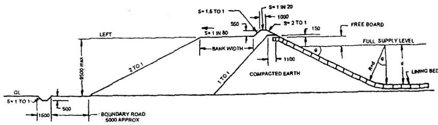
All dimensions in millimetres. FIG. 1A NATURAL GROUND BELOW BED
