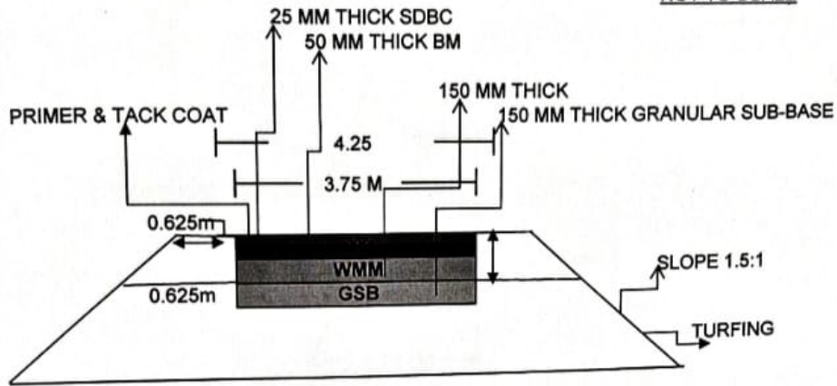
TYPICAL CROSS SECTION OF BT ROAD
