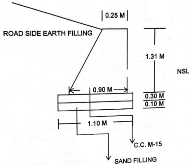
TYPICAL SECTION OF TOE WALL
